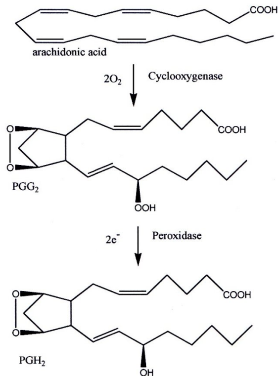
Figure 1.6 Arachidonic acid conversion to PGH 2
